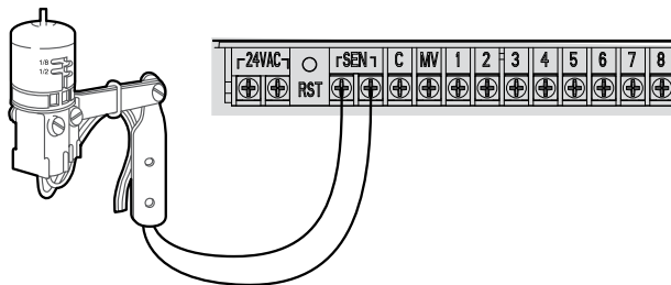
Mini-Clik Rain Sensor
